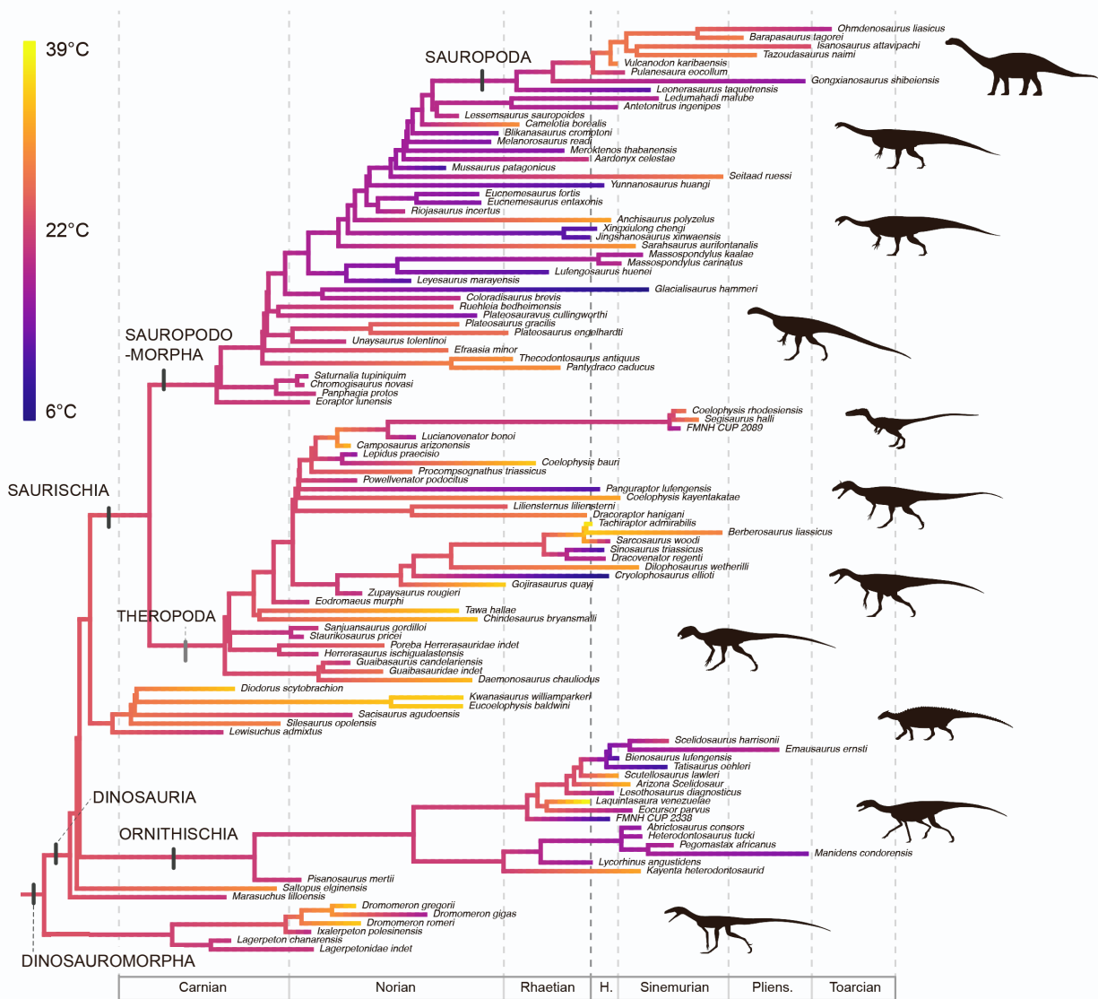
Figure S2: Mean annual temperature (MAT) mapped as a continuous character onto a single timescaled tree. Related to Figure 3. This tree displays the topology of McPhee et al. S1 where polytomies have been randomly resolved as detailed in the STAR Methods. During the early divergences of sauropodomorphs in the Late Triassic inferred climate niches are ‘cooler’. By contrast, in the Early Jurassic Sarhsaurus , Seitaad and sauropods have ‘warmer’ climate niches. Timescale abbreviations: H., Hettangian; Pliens., Pliensbachian. Silhouettes from phylopic.org: Coelophysis by Tasman Dixon, Vulcanodon by Roberto Diaz Sibaja, Eodromaeus by Conty, and Massospondylus , Plateosaurus , Eoraptor , Cryolophosaurus , Scelidosaurus , Silesaurus , and Ixalerpton all by Scott Hartman.
