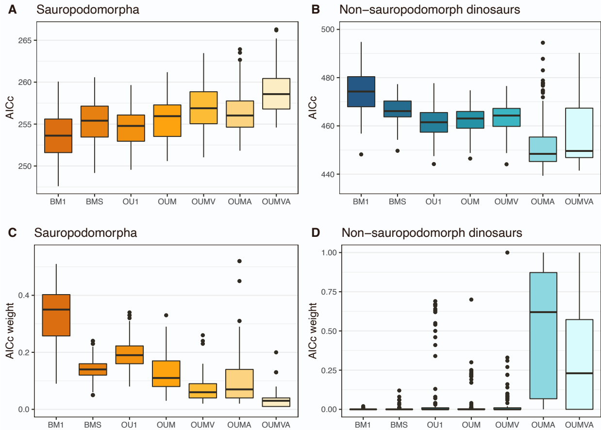
Figure S3: AICc values and weights for evolutionary model fitting analysis. Related to Figure 4. AICc values (a-b) and weights (c-d) for evolutionary model fitting analysis using MAT involving Sauropodomorpha (orange; Chapelle et al. S2 topology) and non-sauropodomorph dinosaurs (blue). Lower AICc values indicate greater support for a model, while higher AICc weights indicate more support. Models beginning “BM” indicate Brownian motion, and those beginning “OU” indicate Ornstein-Uhlenbeck; for full list see Table S3.
